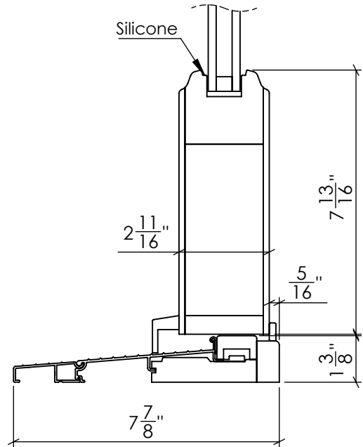
Sill detail D-D
