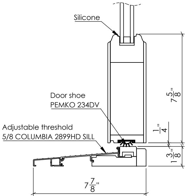
Sill detail C-C
