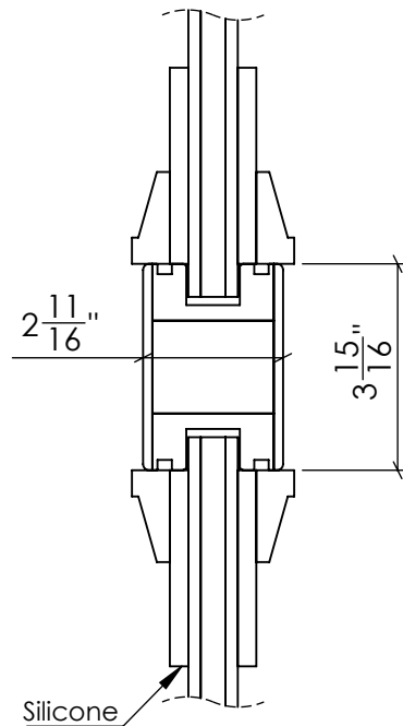
Intermediate Rail C-C
