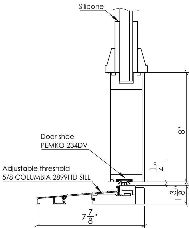
Sill detail C-C
